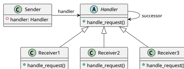
Figure 321: UML Diagram of the Chain of Responsibility Pattern
